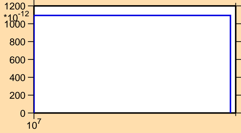
\sigma vs. E for ^{177}\text{Os}(n,pd)
