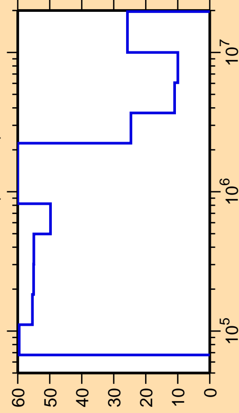
\Delta\sigma/\sigma vs. E for ^{177}\text{Os}(n,\text{inel.})
