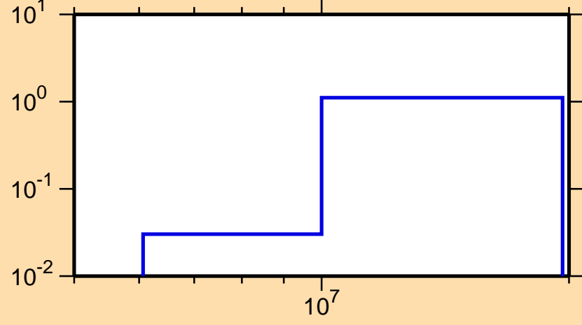
\sigma vs. E for ^{177}\text{Os}(n,2n)
