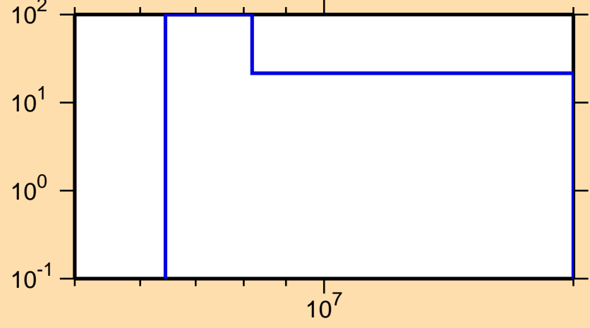
\Delta\sigma/\sigma vs. E for ^{177}\text{Os}(n,2n)
