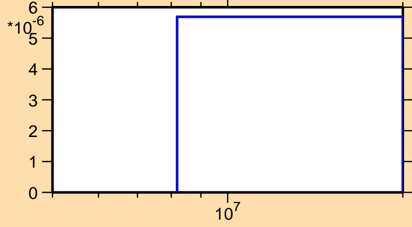
\sigma vs. E for ^{177}\text{Os}(n,2np)
