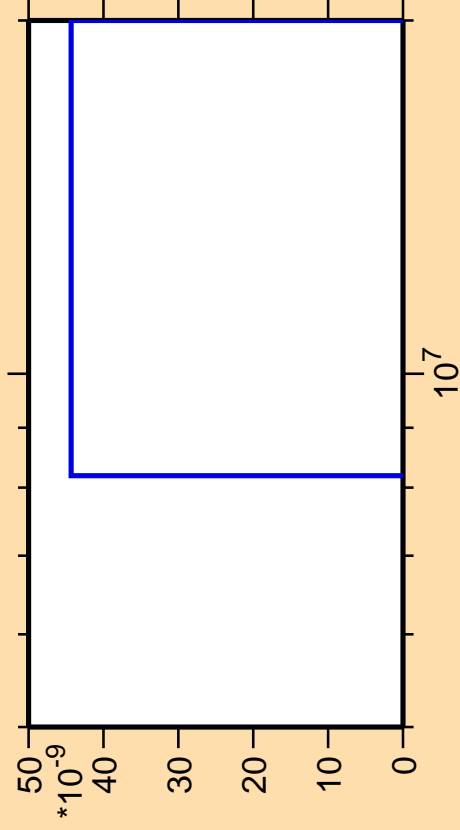
\Delta\sigma/\sigma vs. E for ^{177}\text{Os}(\text{mt } 11)
