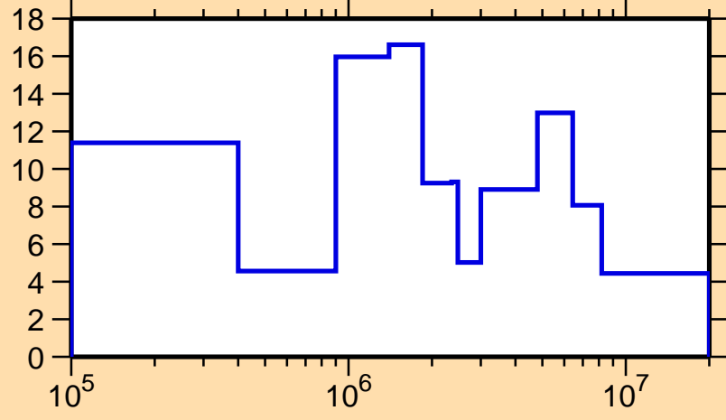
\Delta\sigma/\sigma vs. E for ^{177}\text{Os}(n, el.)
