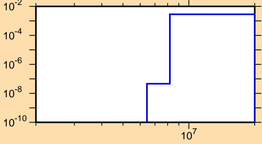
\sigma vs. E for ^{177}\text{Os}(n,d)
