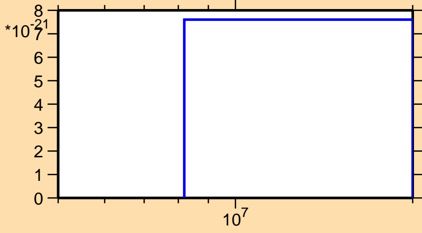
\sigma vs. E for ^{177}\text{Os}(\text{mt } 11)
