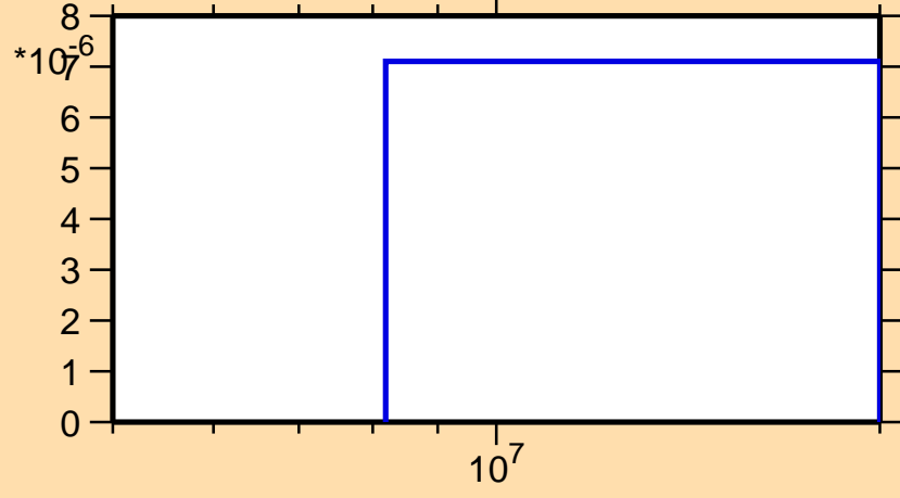
\sigma vs. E for ^{177}\text{Os}(n,3n)
