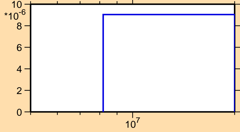
\sigma vs. E for ^{177}\text{Os}(n,2n\alpha)
