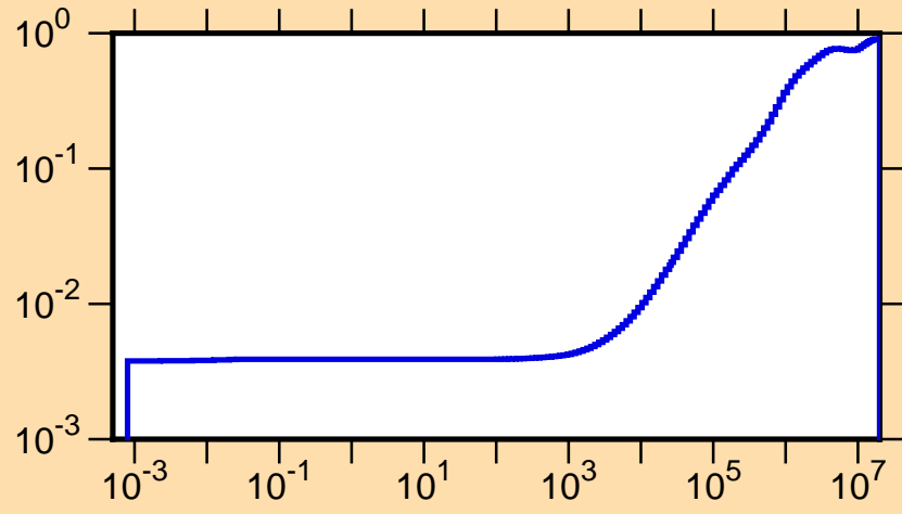
\mu vs. E for ^{178}\text{Os}(\text{mt251})
