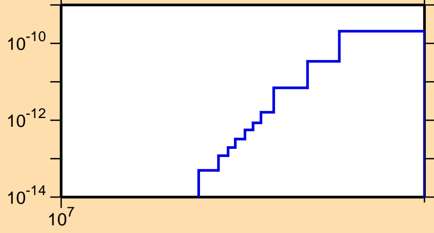
\sigma vs. E for ^{178}\text{Os}(\text{mt117})
