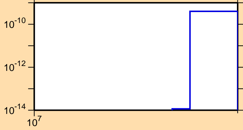
\sigma vs. E for ^{178}\text{Os}(n,nt)
