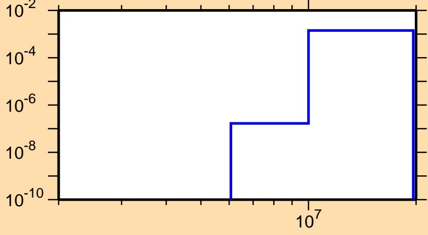
\sigma vs. E for ^{178}\text{Os}(n,d)
