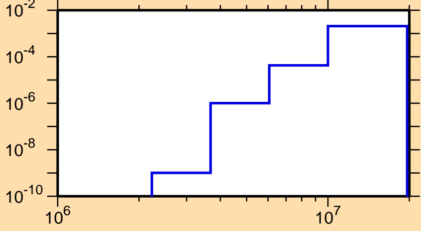
\sigma vs. E for ^{178}\text{Os}(n,n\alpha)
