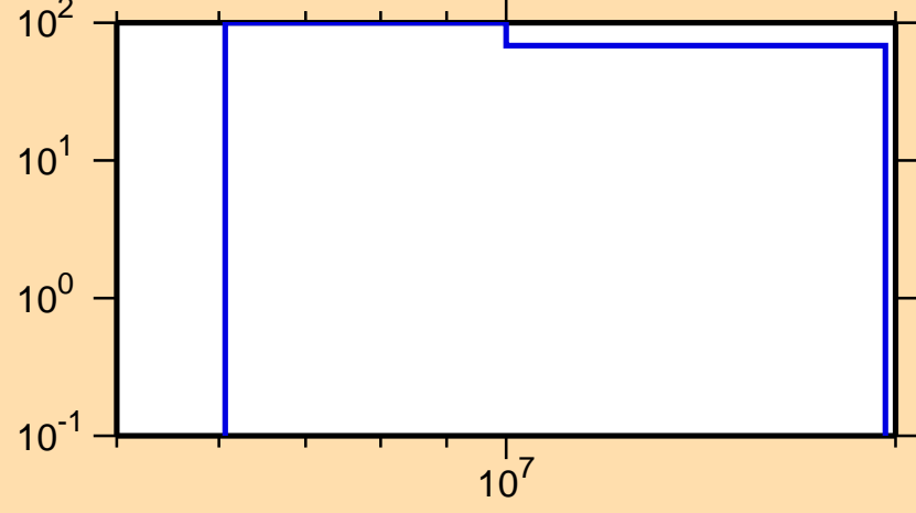
\Delta\sigma/\sigma vs. E for ^{178}\text{Os}(n,2n)
