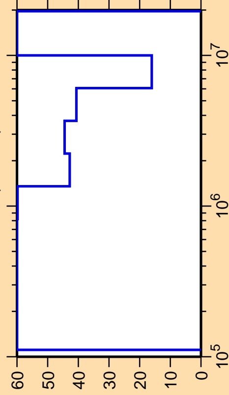
\Delta\sigma/\sigma vs. E for ^{178}\text{Os}(n,\text{inel.})
