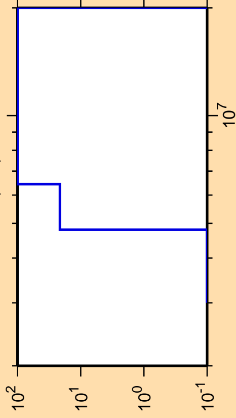
\Delta\sigma/\sigma vs. E for ^{178}\text{Os}(n,d)
