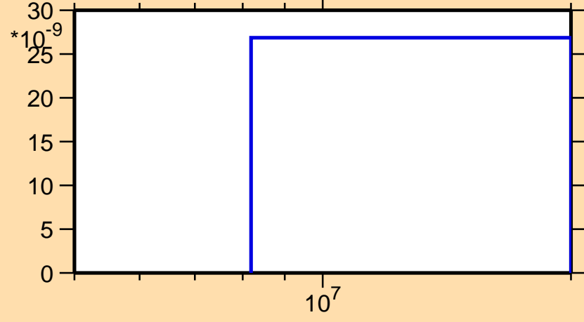
\sigma vs. E for ^{178}\text{Os}(n,2np)
