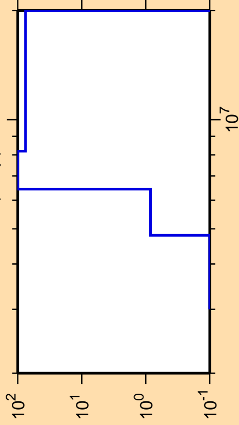
\Delta\sigma/\sigma vs. E for ^{178}\text{Os}(n,np)
