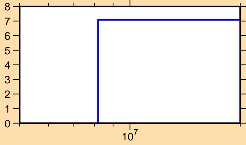
\Delta\sigma/\sigma vs. E for ^{178}\text{Os}(n,\text{el.})
