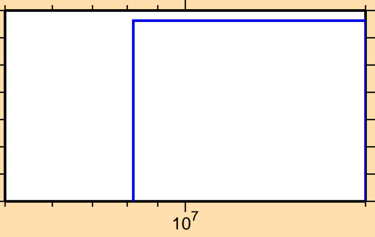
\sigma vs. E for ^{178}\text{Os}(n,\text{He}3)
