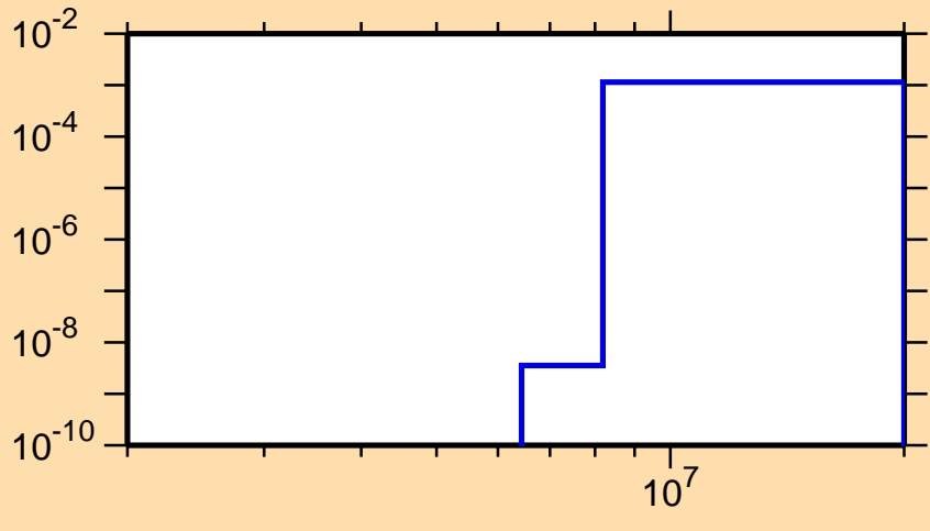
\sigma vs. E for ^{178}\text{Os}(n,d)
