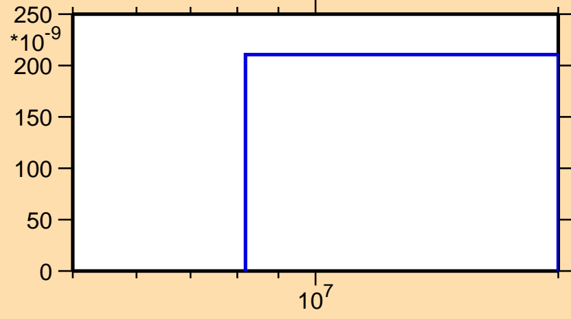
\sigma vs. E for ^{178}\text{Os}(n,2n\alpha)
