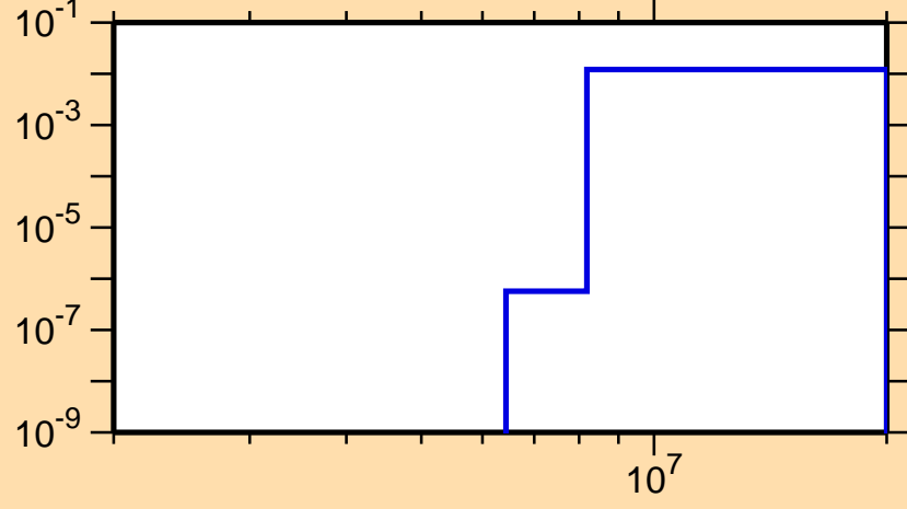
\sigma vs. E for ^{178}\text{Os}(n,np)
