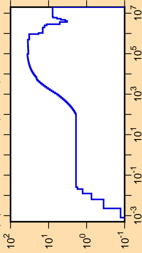
\Delta\mu/\mu vs. E for ^{179}\text{Os}(\text{mt251})
