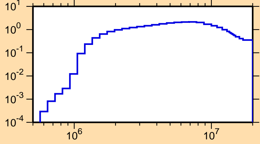
\sigma vs. E for ^{179}\text{Os}(n,n\text{cont.})
