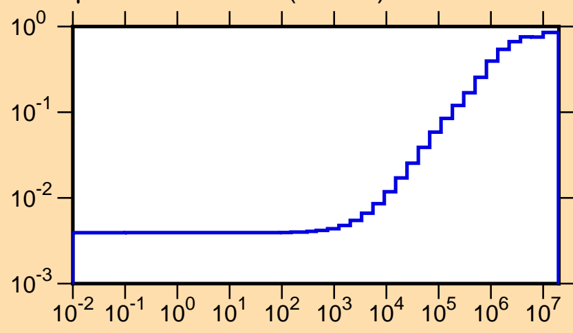
\mu vs. E for ^{179}\text{Os}(\text{mt251})
