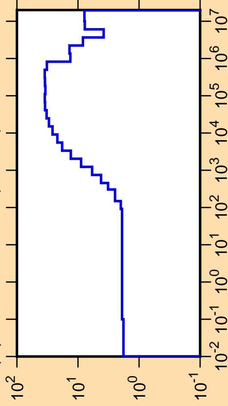
\Delta\mu/\mu vs. E for ^{179}\text{Os}(\text{mt251})
