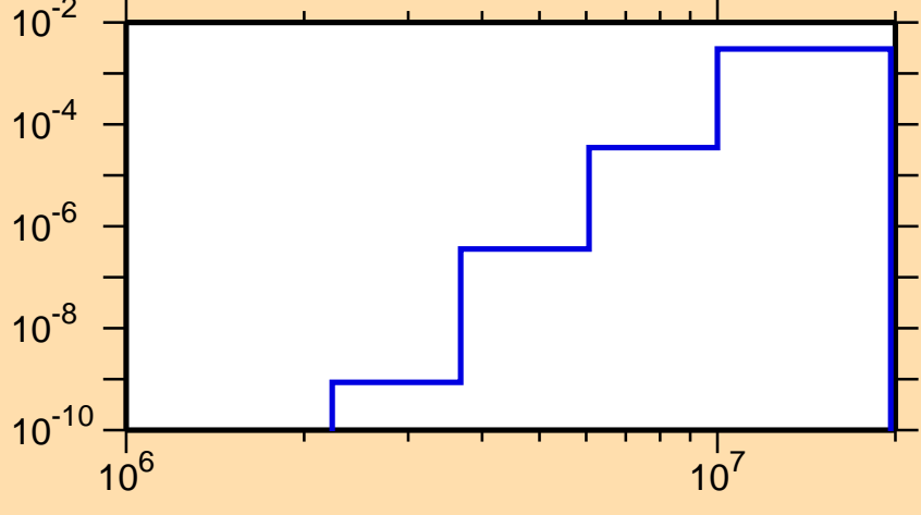
\sigma vs. E for ^{179}\text{Os}(n,n\alpha)
