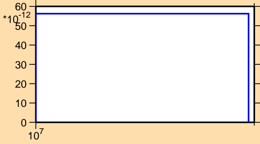
\sigma vs. E for ^{179}\text{Os}(n,pd)
