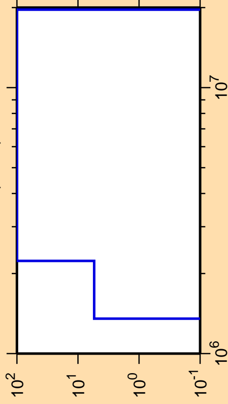
\Delta\sigma/\sigma vs. E for ^{179}\text{Os}(n,n\alpha)
