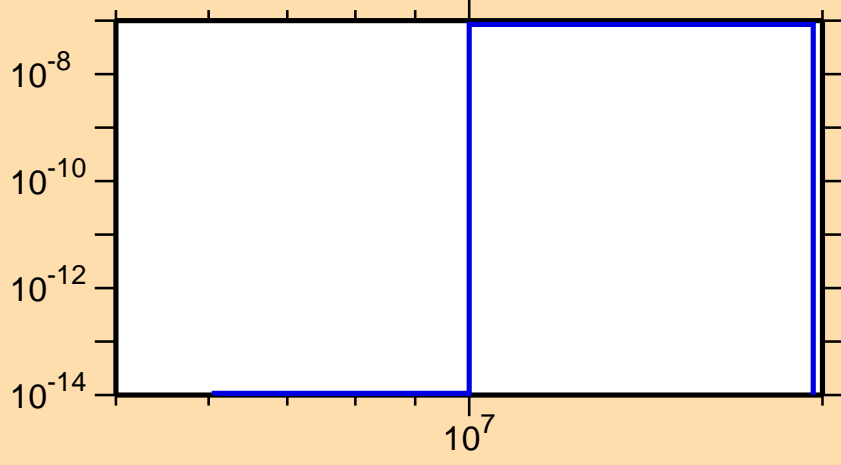
\sigma vs. E for ^{179}\text{Os}(n,\text{He}3)
