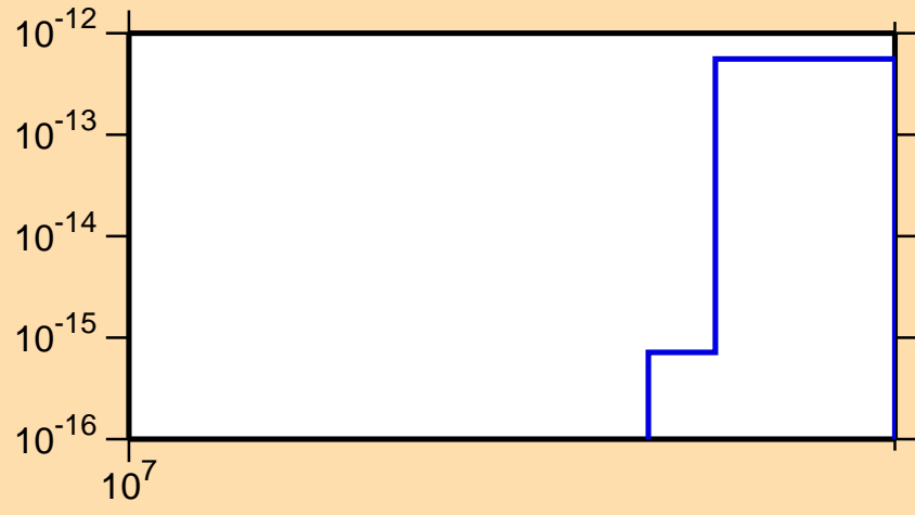
\sigma vs. E for ^{180}\text{Os} (mt 34)
