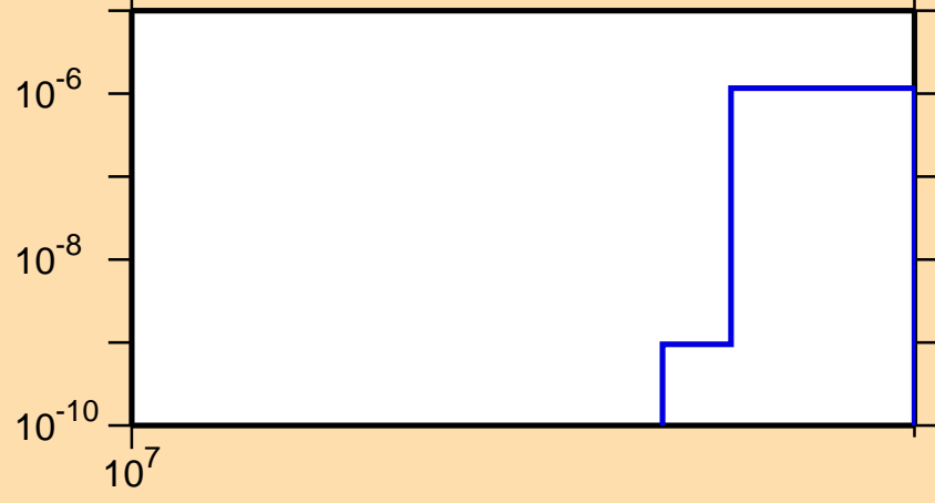
\sigma vs. E for ^{180}\text{Os}(n,2np)
