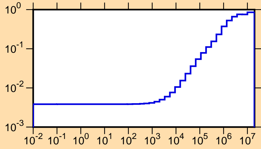
\mu vs. E for ^{180}\text{Os}(\text{mt251})
