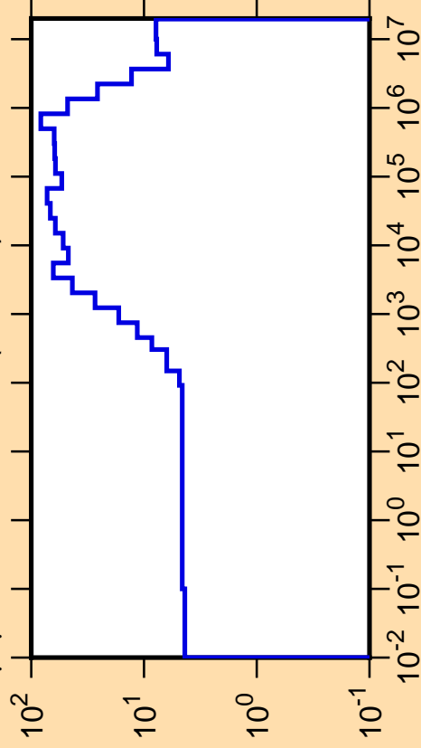
\Delta\mu/\mu vs. E for ^{180}\text{Os}(\text{mt251})
