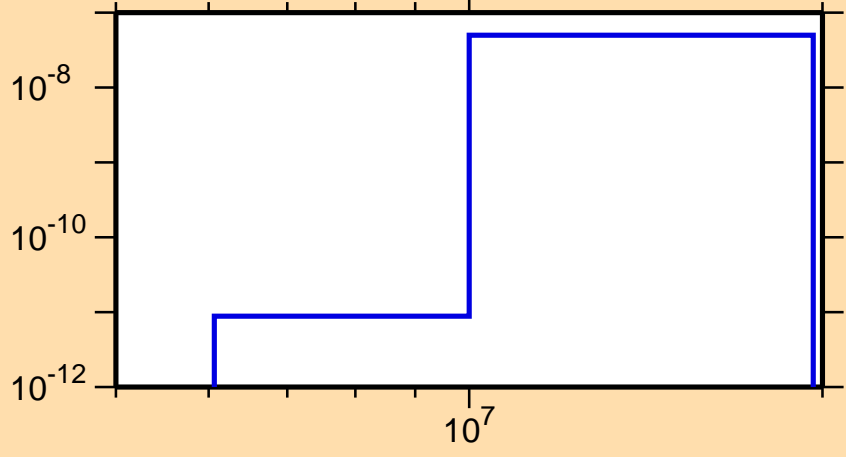
\sigma vs. E for ^{180}\text{Os}(n,p\alpha)
