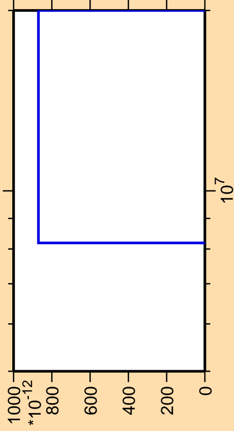
\Delta\sigma/\sigma vs. E for ^{180}\text{Os}(\text{mt } 11)
