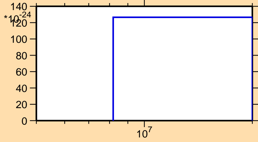
\sigma vs. E for ^{180}\text{Os}(\text{mt } 11)
