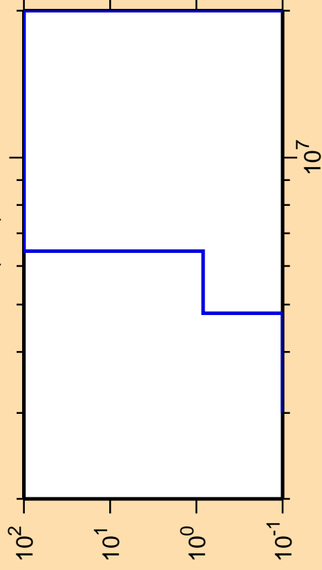
\Delta\sigma/\sigma vs. E for ^{180}\text{Os}(n,d)
