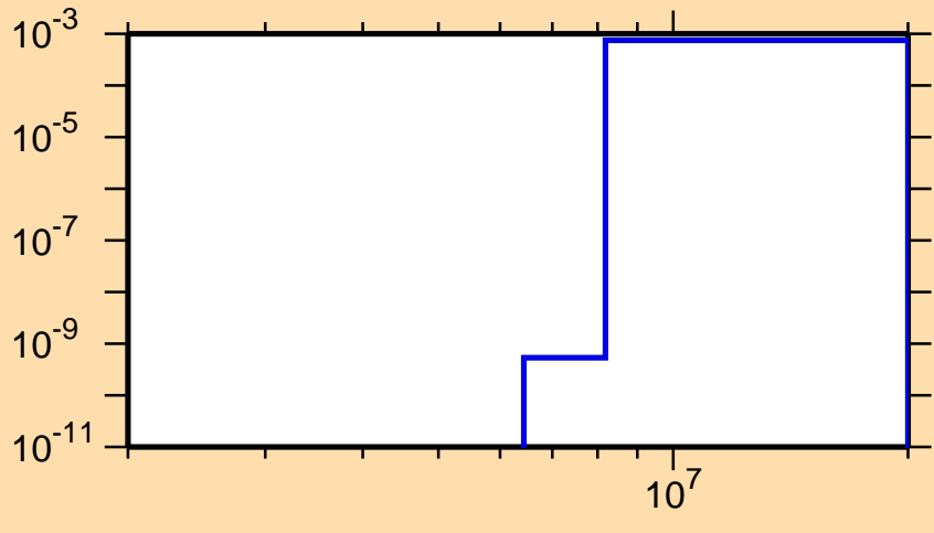
\sigma vs. E for ^{180}\text{Os}(n,d)
