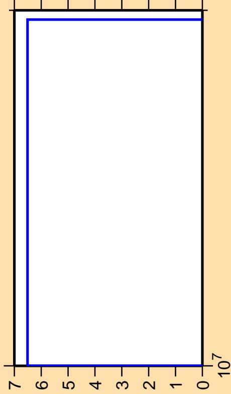
\Delta\sigma/\sigma vs. E for ^{181}\text{Os}(n,\text{pd})
