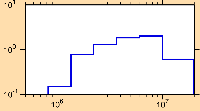
\sigma vs. E for ^{181}\text{Os}(n,n\text{cont.})
