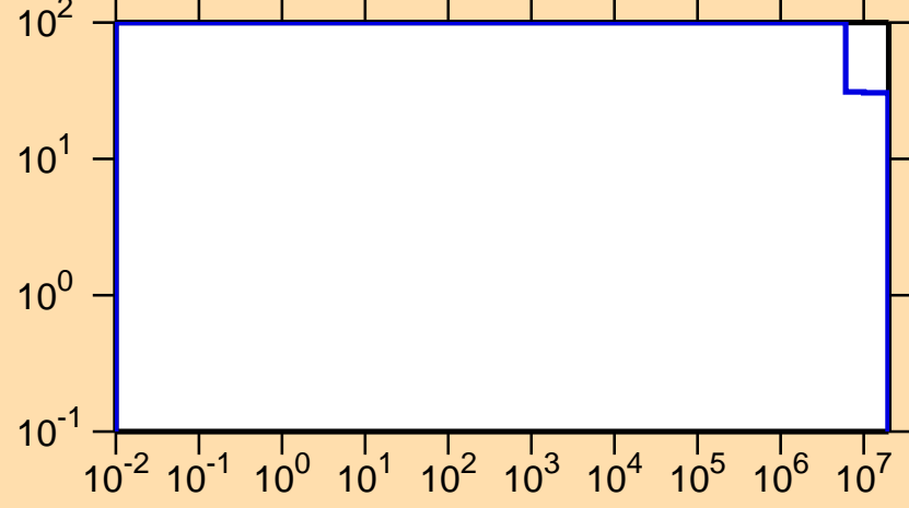
\Delta\sigma/\sigma vs. E for ^{181}\text{Os}(n,p)
