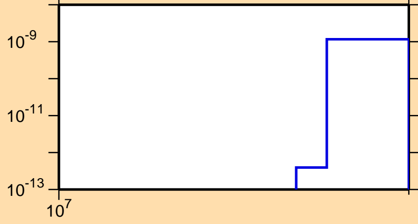
\sigma vs. E for ^{181}\text{Os}(n,nt)
