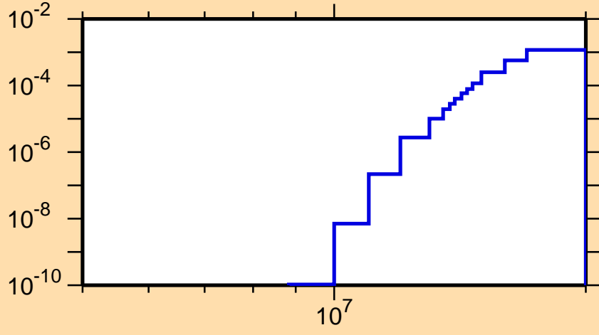
\sigma vs. E for ^{181}\text{Os}(n,t)
