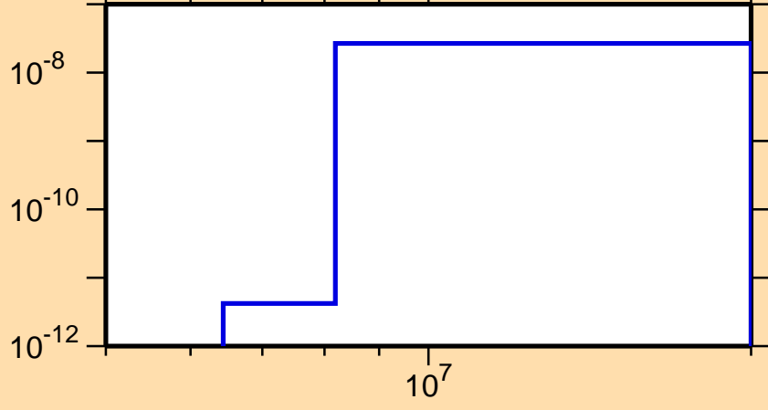
\sigma vs. E for ^{181}\text{Os}(n,p\alpha)
