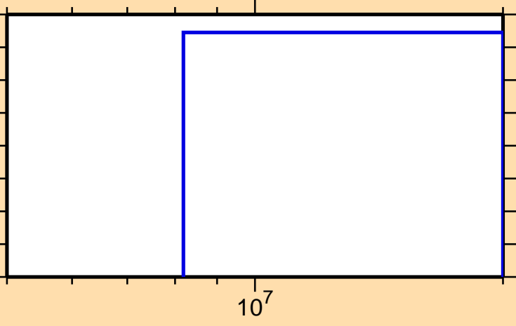
\sigma vs. E for ^{181}\text{Os}(n,2n\alpha)
