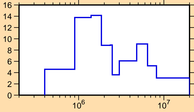
\Delta\sigma/\sigma vs. E for ^{181}\text{Os}(n, el.)
