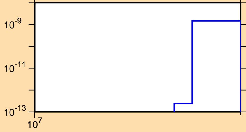
\sigma vs. E for ^{182}\text{Os}(n,nt)
