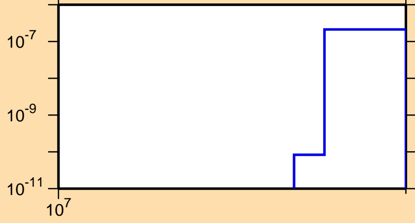
\sigma vs. E for ^{182}\text{Os}(n,2np)
