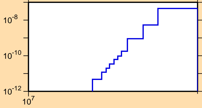
\sigma vs. E for ^{182}\text{Os}(n,\text{He}3)
