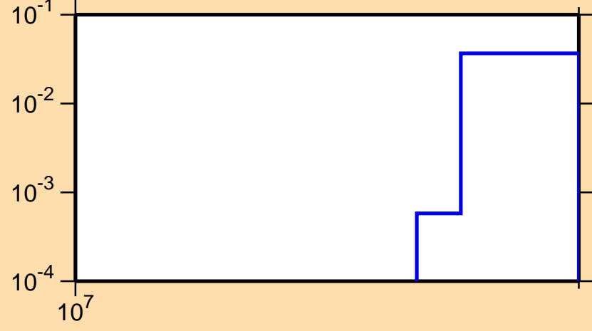
\sigma vs. E for ^{182}\text{Os}(n,3n)
