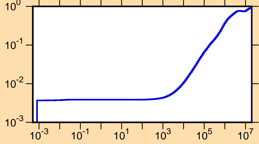
\mu vs. E for ^{183}\text{Os}(\text{mt251})
