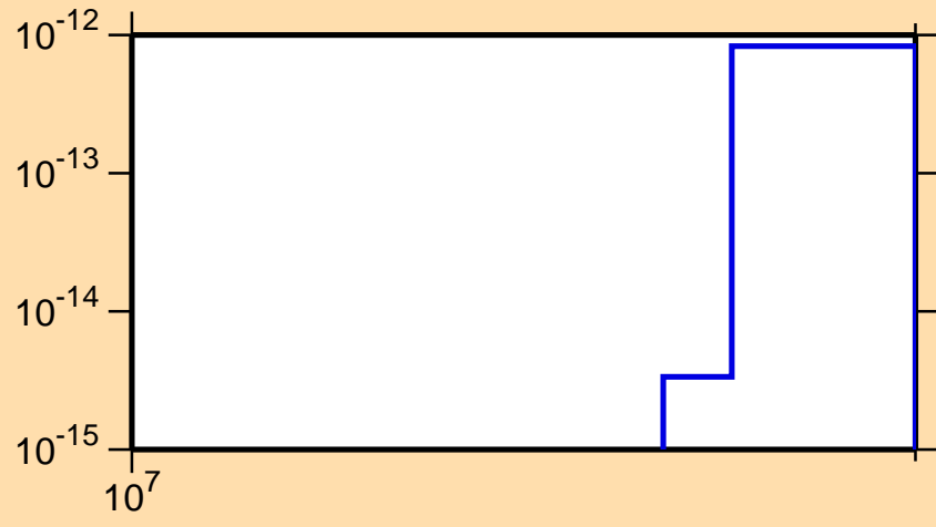
\sigma vs. E for ^{183}\text{Os}(n,\text{pt})
