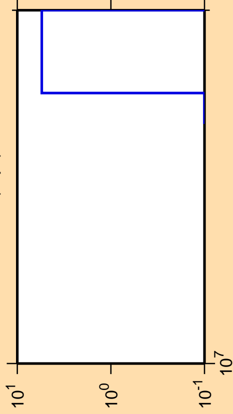
\Delta\sigma/\sigma vs. E for ^{183}\text{Os}(n,\text{pt})
