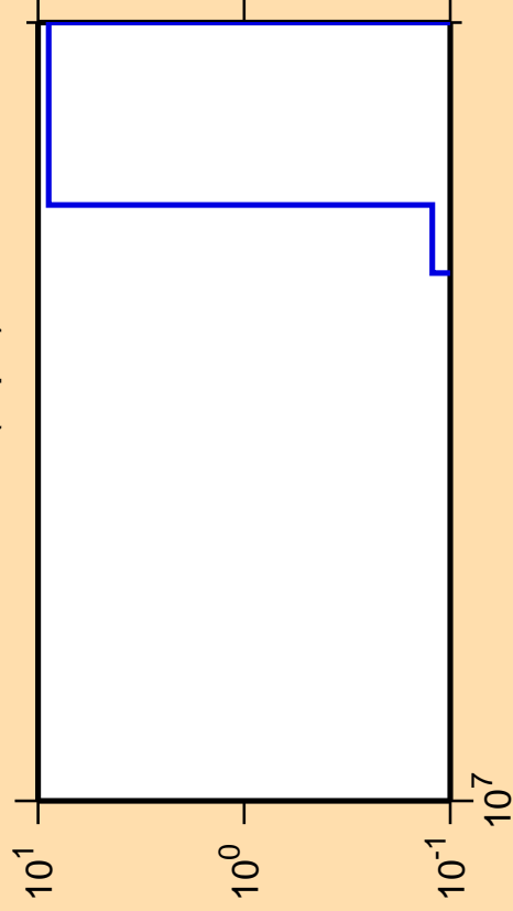
\Delta\sigma/\sigma vs. E for ^{183}\text{Os}(n,\text{pd})
