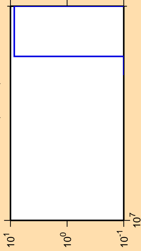
\Delta\sigma/\sigma vs. E for ^{183}\text{Os} (mt 34)
