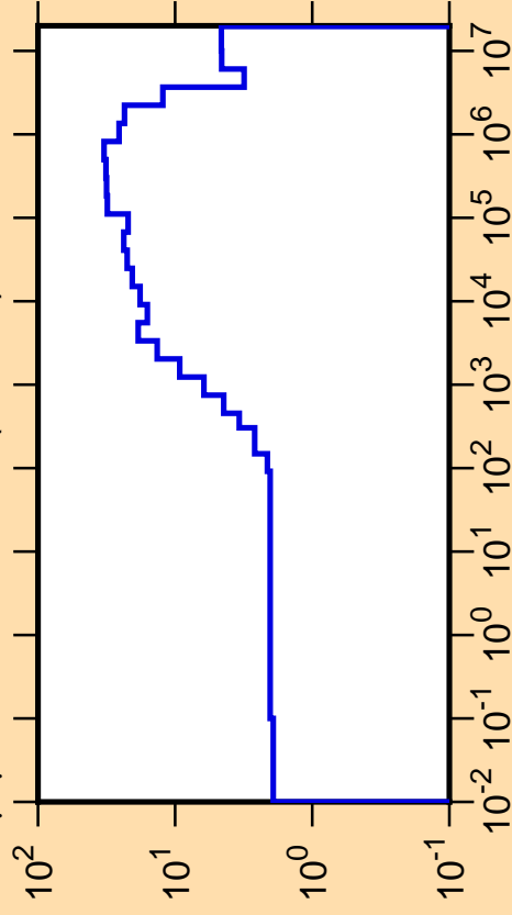
\Delta\mu/\mu vs. E for ^{183}\text{Os}(\text{mt251})
