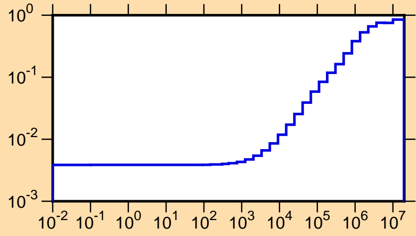
\mu vs. E for ^{183}\text{Os}(\text{mt251})
