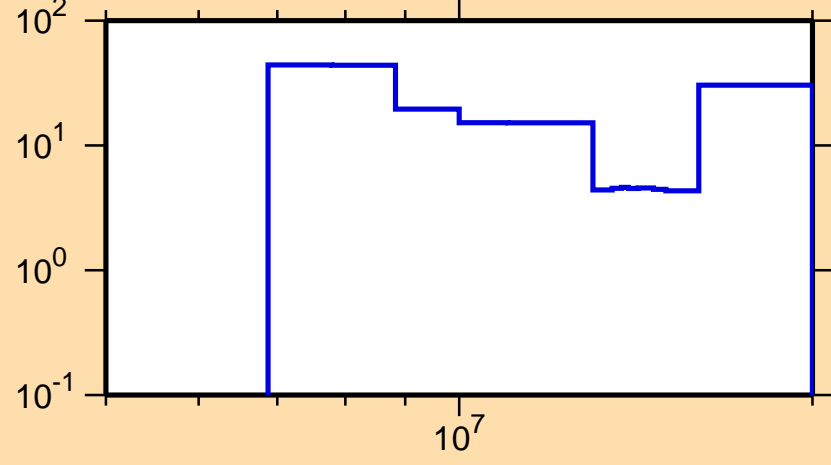
\Delta\sigma/\sigma vs. E for ^{183}\text{Os}(n,2n)
