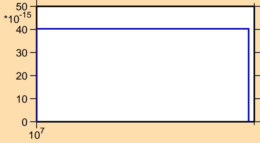
\sigma vs. E for ^{183}\text{Os}(n,pd)
