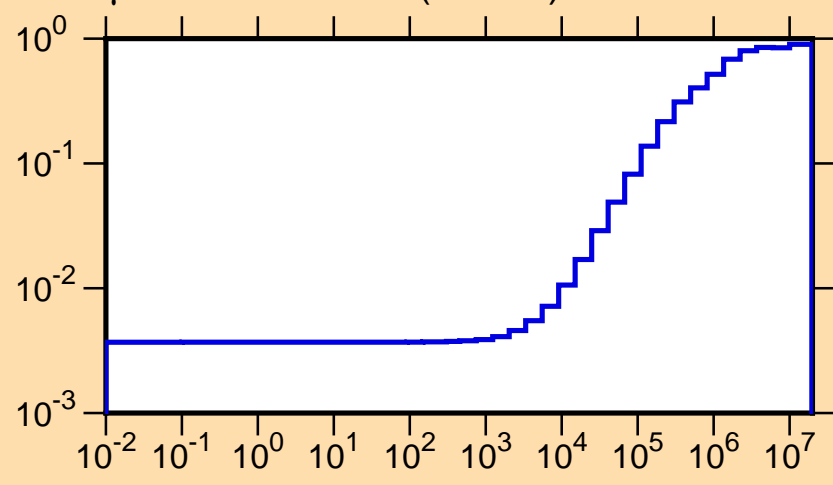
\mu vs. E for ^{184}\text{Os}(\text{mt251})
