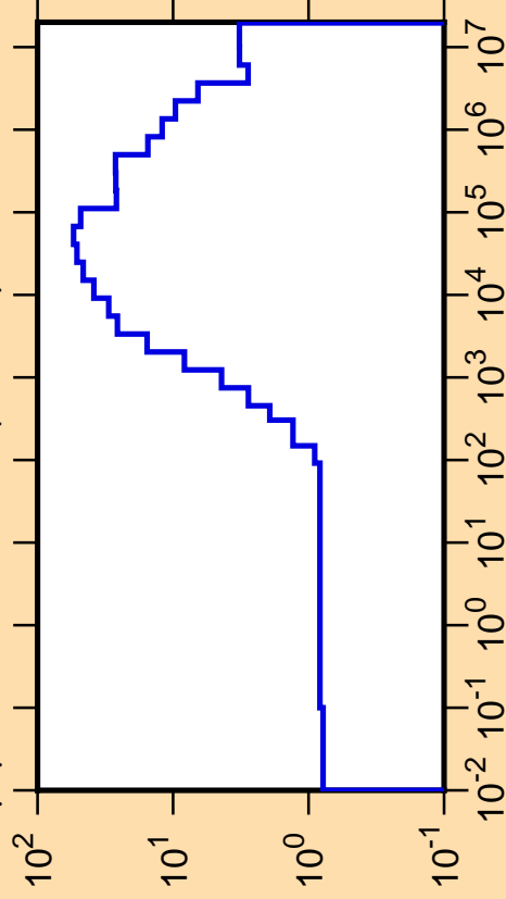
\Delta\mu/\mu vs. E for ^{184}\text{Os}(\text{mt251})
