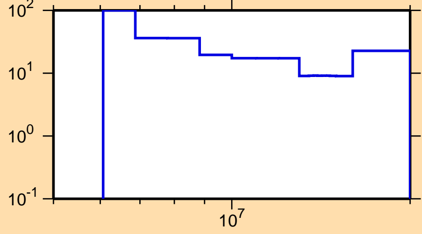
\Delta\sigma/\sigma vs. E for ^{185}\text{Os}(n,2n)
