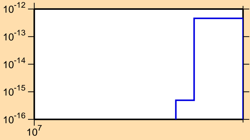
\sigma vs. E for ^{185}\text{Os} (mt 34)
