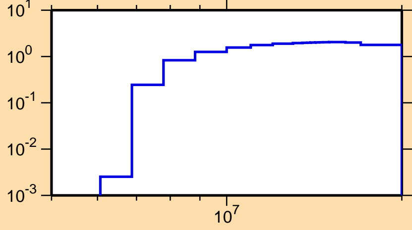
\sigma vs. E for ^{185}\text{Os}(n,2n)
