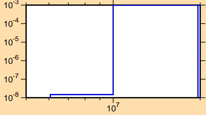
\sigma vs. E for ^{185}\text{Os}(n,d)
