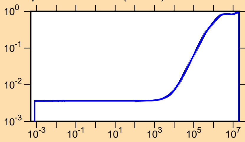
\mu vs. E for ^{186}\text{Os}(\text{mt251})
