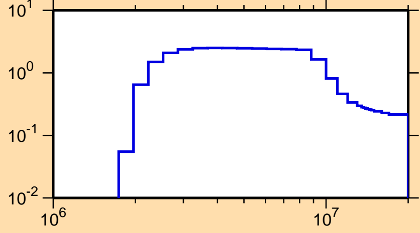
\sigma vs. E for ^{186}\text{Os}(n,n\text{cont.})
