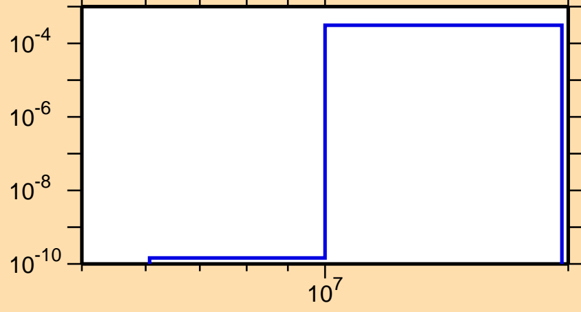
\sigma vs. E for ^{186}\text{Os}(n,np)
