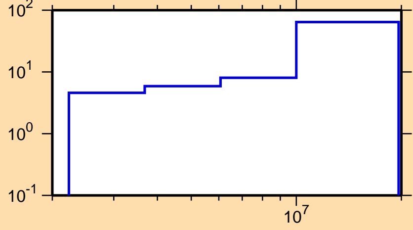
\Delta\sigma/\sigma vs. E for ^{186}\text{Os}(n,n\text{cont.})
