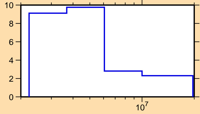
\Delta\sigma/\sigma vs. E for ^{186}\text{Os}(n,el.)
