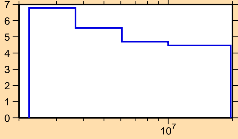
\Delta\sigma/\sigma vs. E for ^{186}\text{Os}(n,\text{nonel.})
