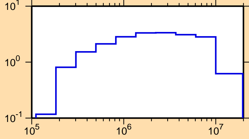
\sigma vs. E for ^{186}\text{Os}(n,\text{inel.})
