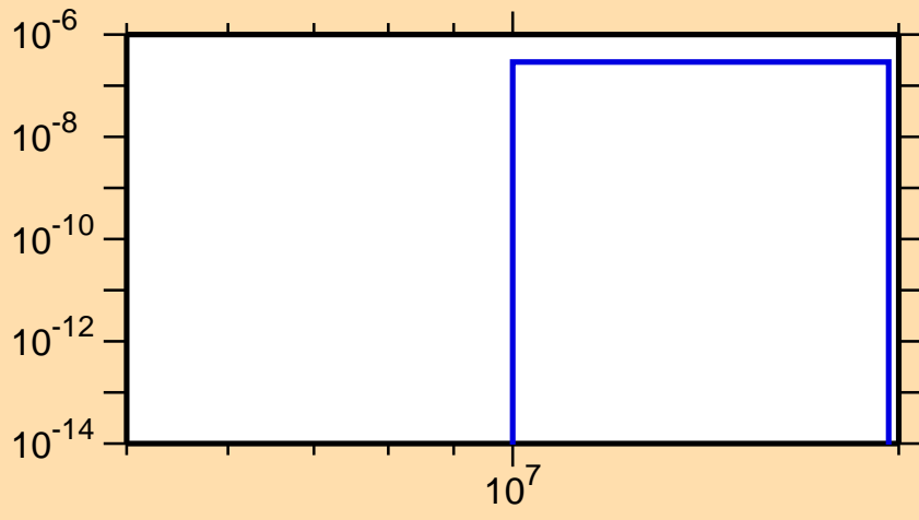
\sigma vs. E for ^{187}\text{Os}(n,2n\alpha)
