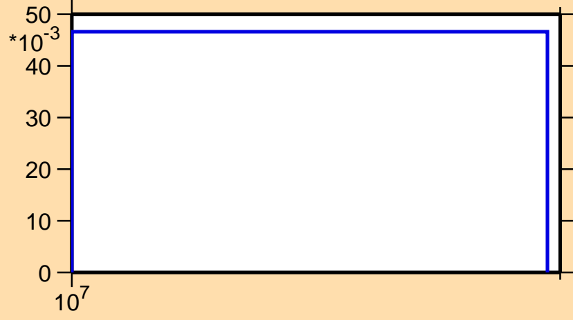
\sigma vs. E for ^{187}\text{Os}(n,3n)
