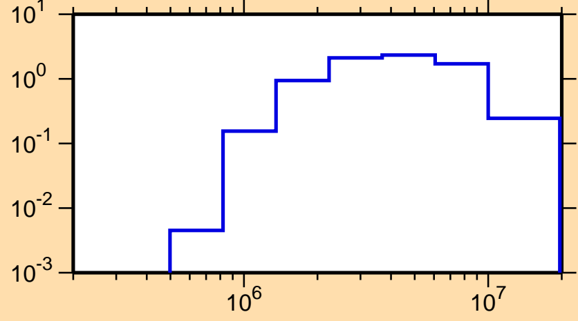
\sigma vs. E for ^{187}\text{Os}(n,n\text{cont.})
