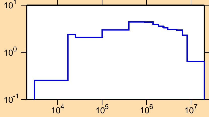
\sigma vs. E for ^{187}\text{Os}(n,\text{inel.})
