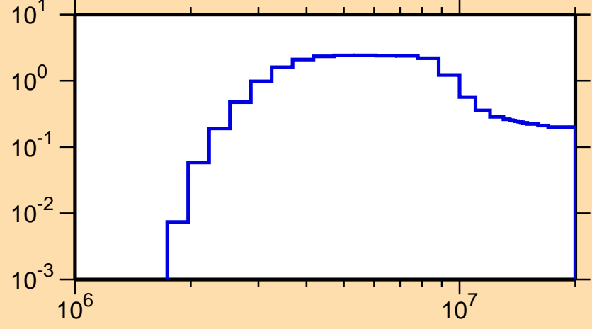
\sigma vs. E for ^{188}\text{Os}(n,n\text{cont.})
