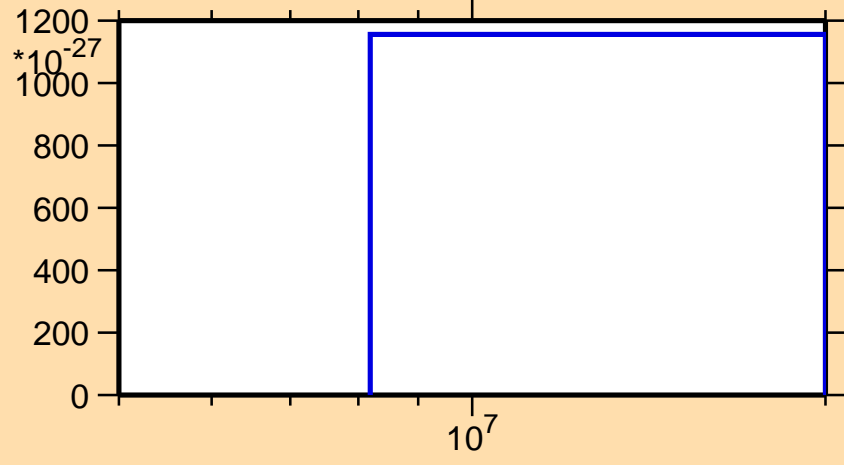
\sigma vs. E for ^{188}\text{Os}(\text{mt } 11)
