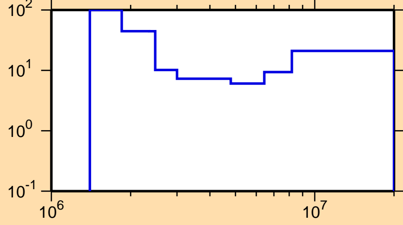
\Delta\sigma/\sigma vs. E for ^{188}\text{Os}(n,n\text{cont.})
