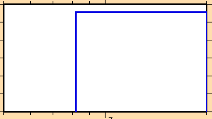
\sigma vs. E for ^{188}\text{Os}(n,nt)
