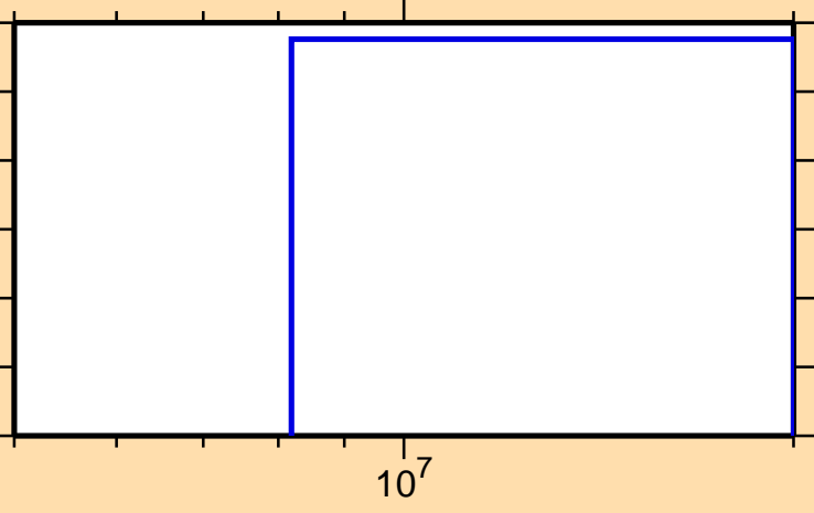
\sigma vs. E for ^{188}\text{Os}(n,3n)
