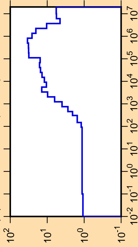
\Delta\mu/\mu vs. E for ^{189}\text{Os}(\text{mt251})
