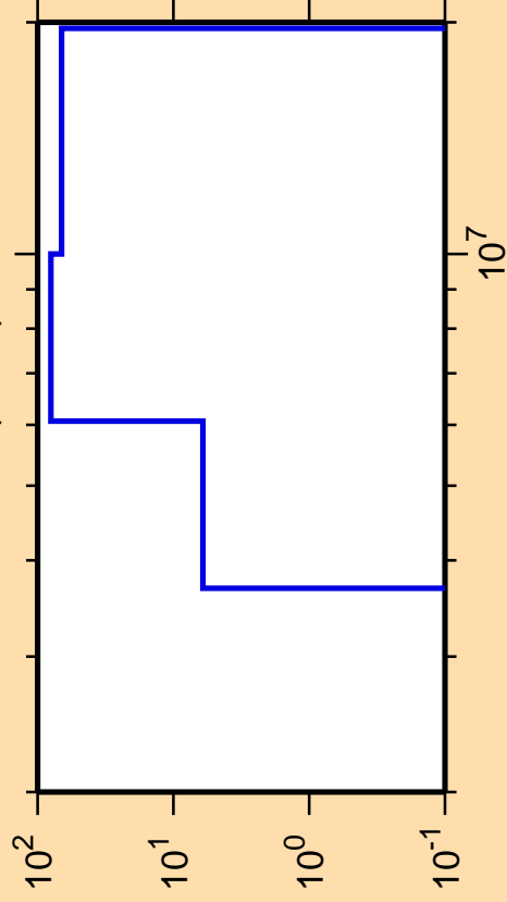
\Delta\sigma/\sigma vs. E for ^{189}\text{Os}(n,n\alpha)
