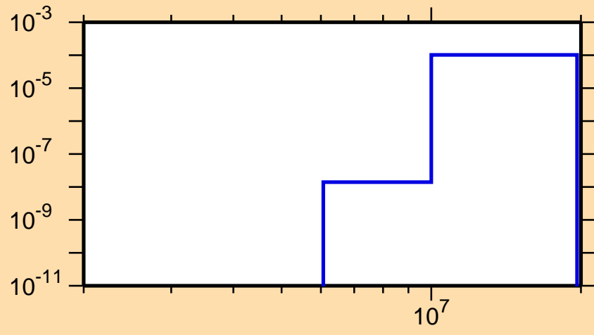
\sigma vs. E for ^{189}\text{Os}(n,n\alpha)
