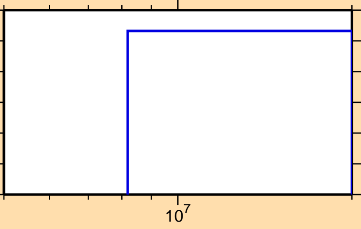
\sigma vs. E for ^{189}\text{Os}(n,3n)
