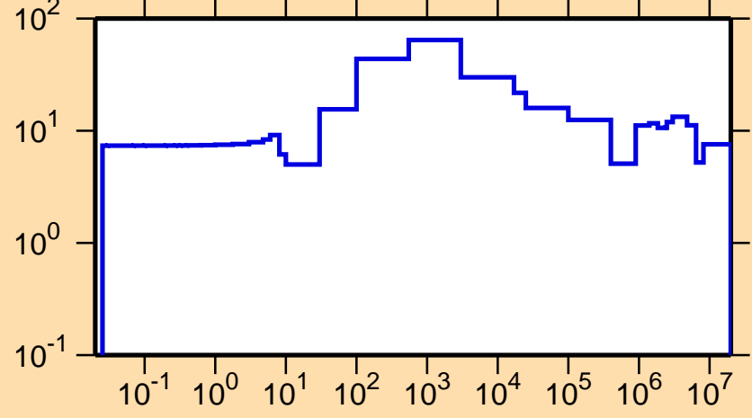
\Delta\sigma/\sigma vs. E for ^{189}\text{Os}(n,\text{el.})
