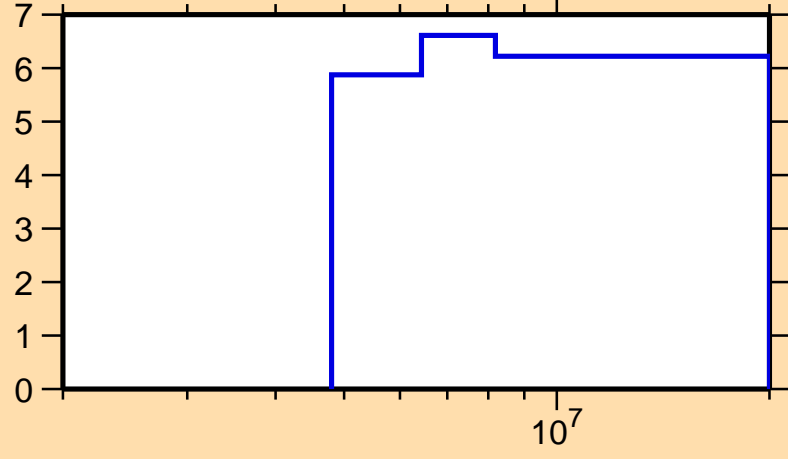
\Delta\sigma/\sigma vs. E for ^{189}\text{Os}(n,\text{nonel.})
