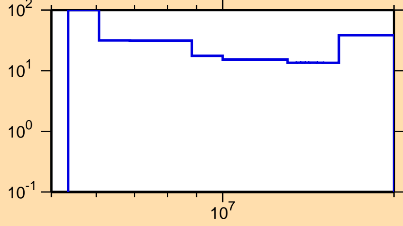
\Delta\sigma/\sigma vs. E for ^{189}\text{Os}(n,2n)
