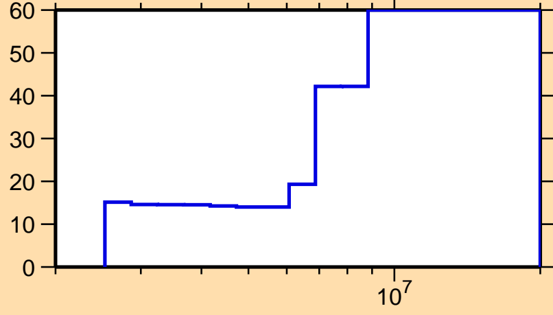
\Delta\sigma/\sigma vs. E for ^{189}\text{Os}(n,ncont.)
