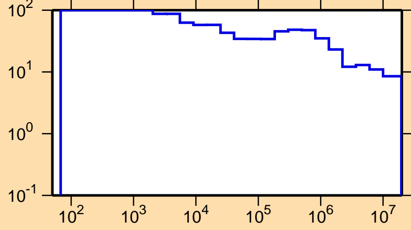
\Delta\sigma/\sigma vs. E for ^{189}\text{Os}(n,\text{nonel.})
