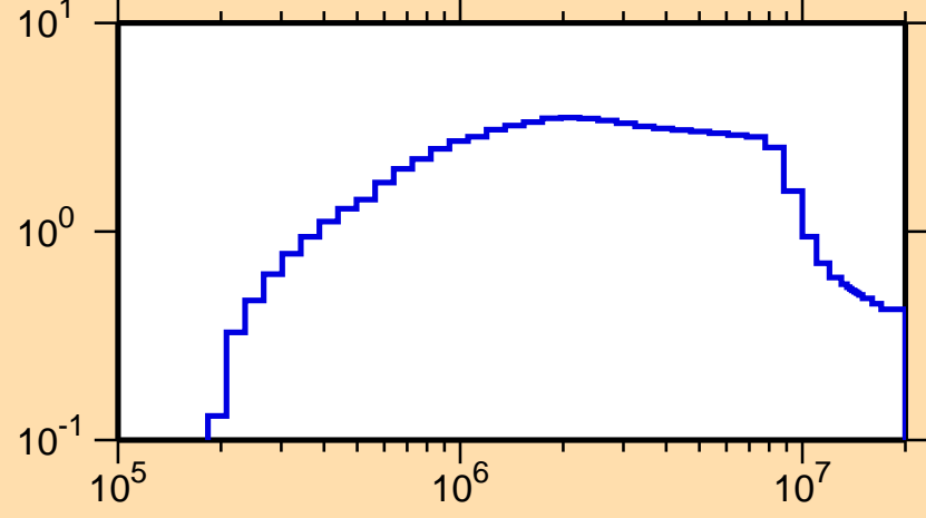
\sigma vs. E for ^{190}\text{Os}(n,\text{inel.})
