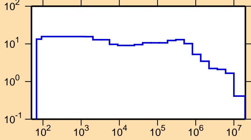
\Delta\sigma/\sigma vs. E for ^{190}\text{Os}(n,\text{tot.})
