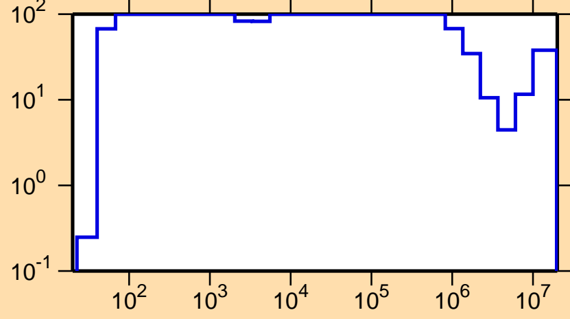
\Delta\sigma/\sigma vs. E for ^{190}\text{Os}(n,n\text{cont.})
