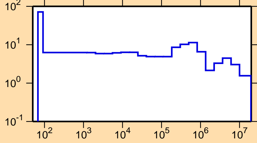
\Delta\sigma/\sigma vs. E for ^{190}\text{Os}(n,\text{el.})
