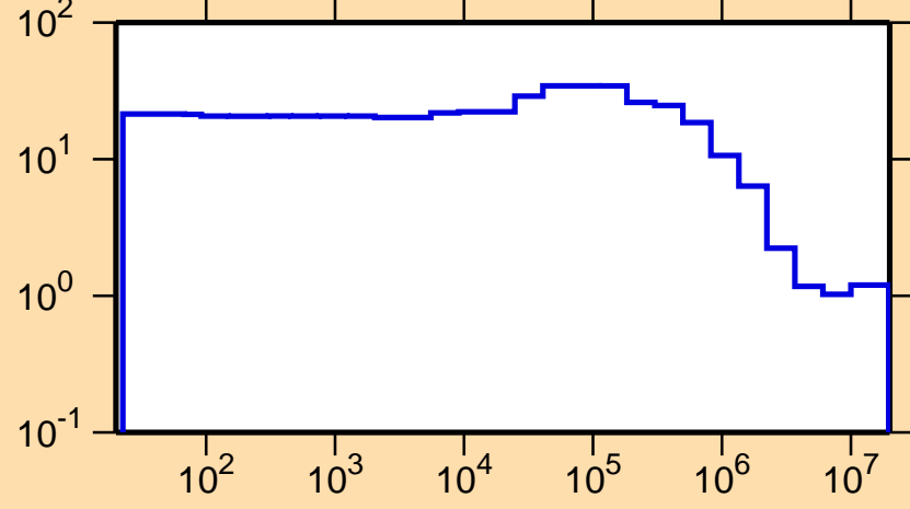
\Delta\sigma/\sigma vs. E for ^{190}\text{Os}(n,\text{nonel.})
