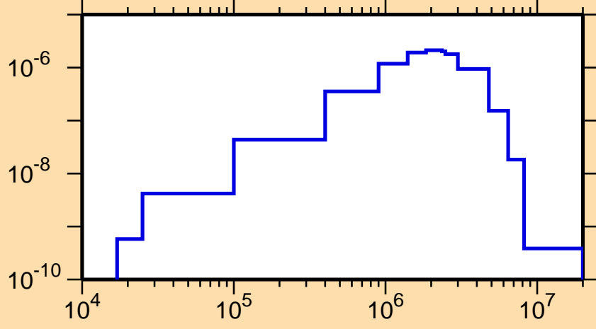
\sigma vs. E for ^{190}\text{Os}(n,n_1)
