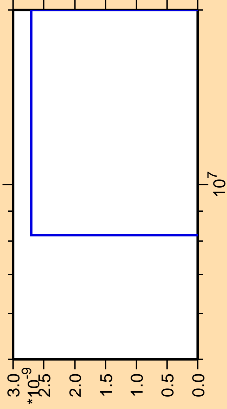
\Delta\sigma/\sigma vs. E for ^{190}\text{Os} (mt 42)
