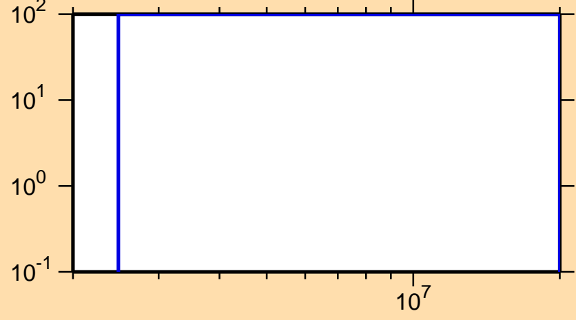
\Delta\sigma/\sigma vs. E for ^{190}\text{Os}(n,n_1)
