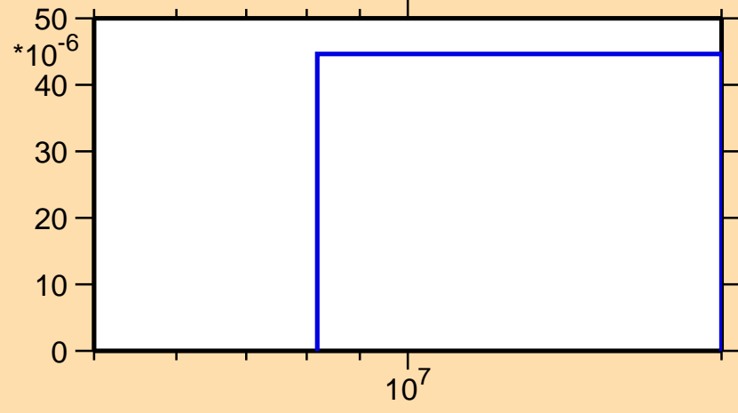
\sigma vs. E for ^{190}\text{Os}(n,np)
