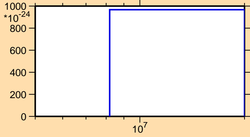
\sigma vs. E for ^{190}\text{Os} (mt 42)
