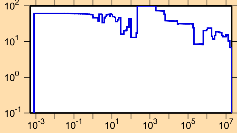
\Delta\sigma/\sigma vs. E for ^{191}\text{Os}(n,\text{el.})
