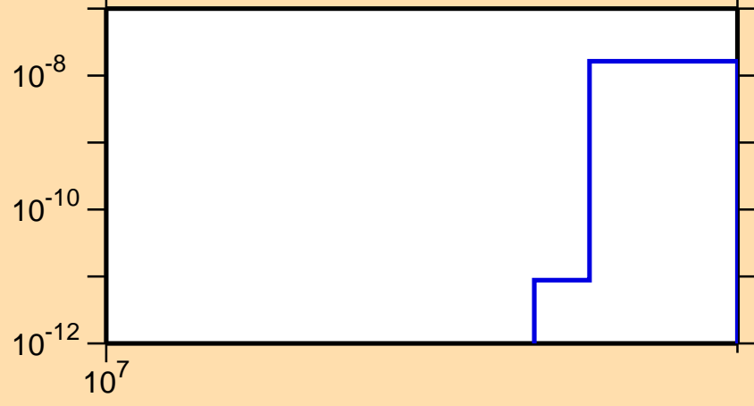
\sigma vs. E for ^{191}\text{Os}(n,nt)
