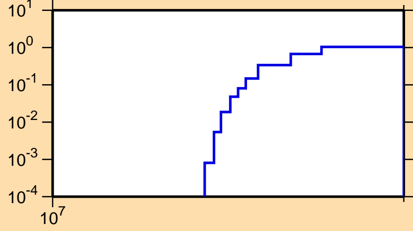
\sigma vs. E for ^{191}\text{Os}(n,3n)
