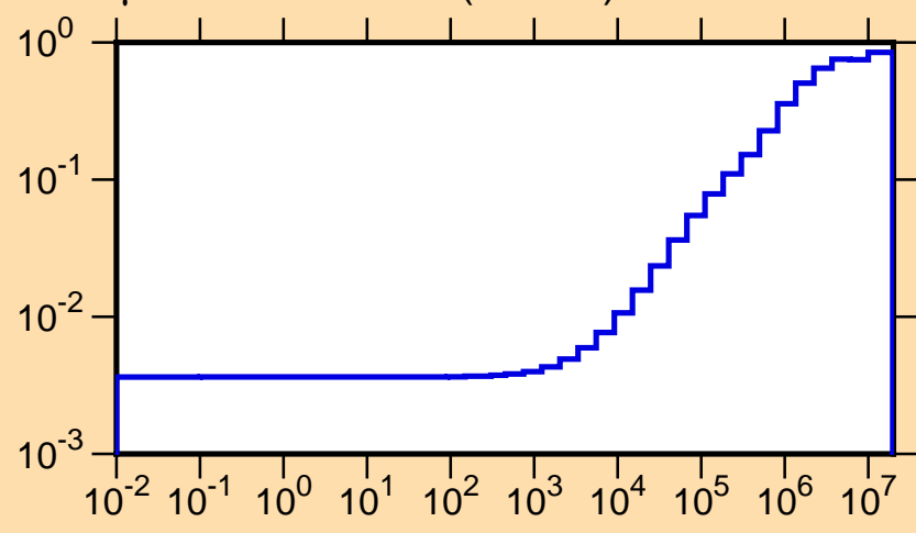
\mu vs. E for ^{191}\text{Os}(\text{mt251})
