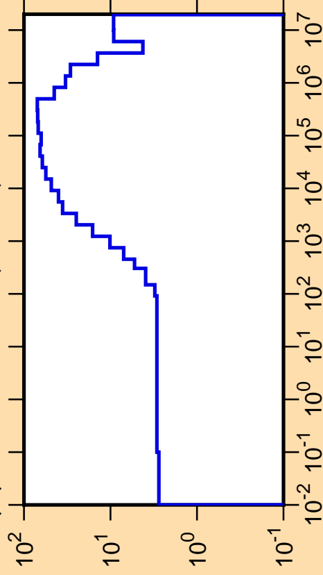
\Delta\mu/\mu vs. E for ^{191}\text{Os}(\text{mt251})
