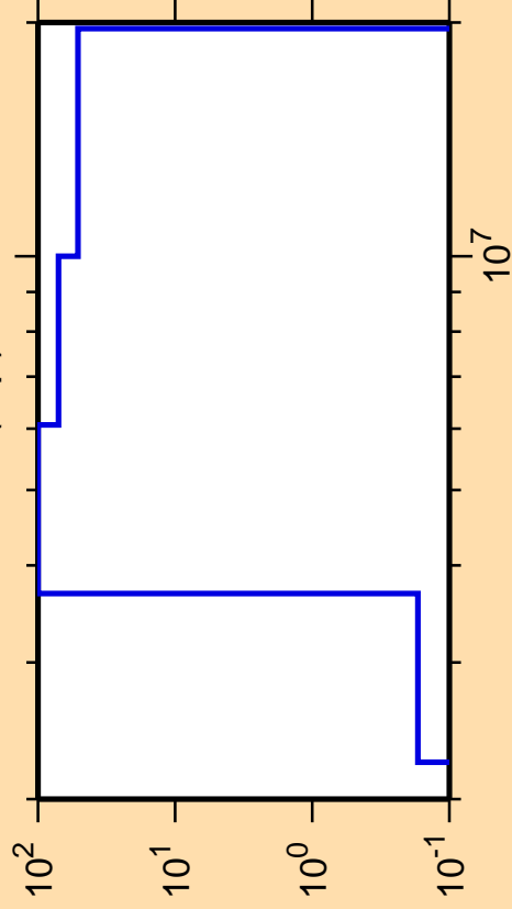
\Delta\sigma/\sigma vs. E for ^{191}\text{Os}(n,p)
