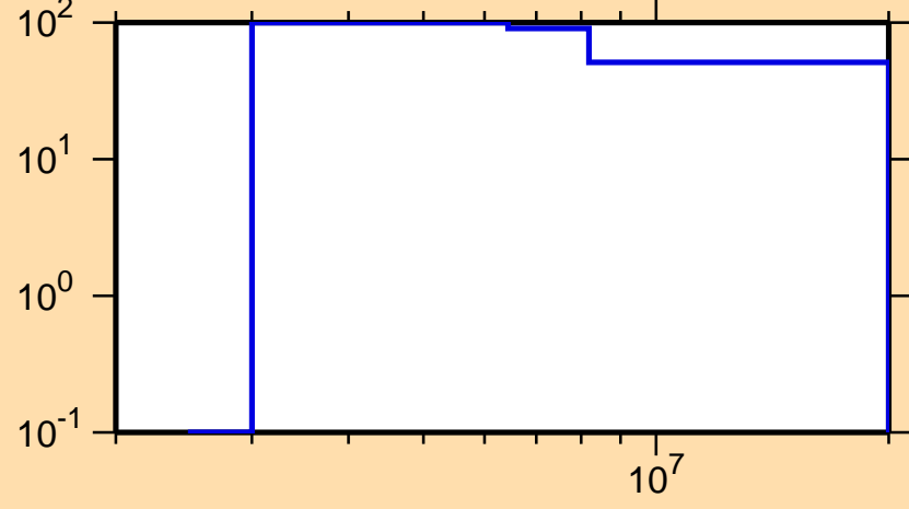
\Delta\sigma/\sigma vs. E for ^{191}\text{Os}(n,p)
