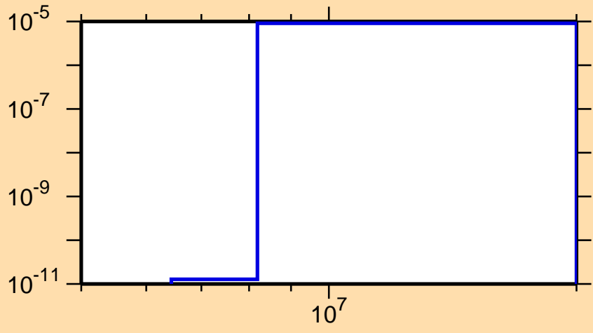
\sigma vs. E for ^{191}\text{Os}(n,n\alpha)
