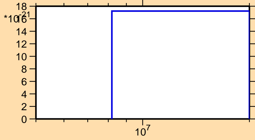
\sigma vs. E for ^{191}\text{Os}(\text{mt } 11)
