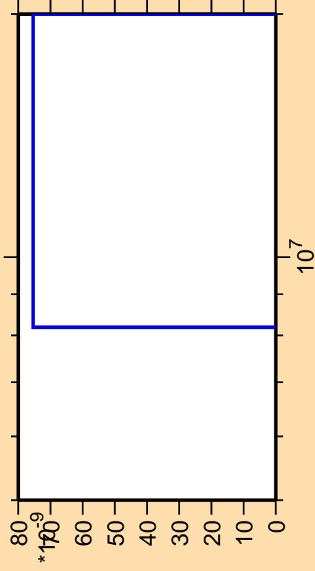
\Delta\sigma/\sigma vs. E for ^{191}\text{Os}(\text{mt } 11)
