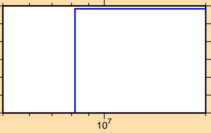
\sigma vs. E for ^{191}\text{Os}(n,2n\alpha)
