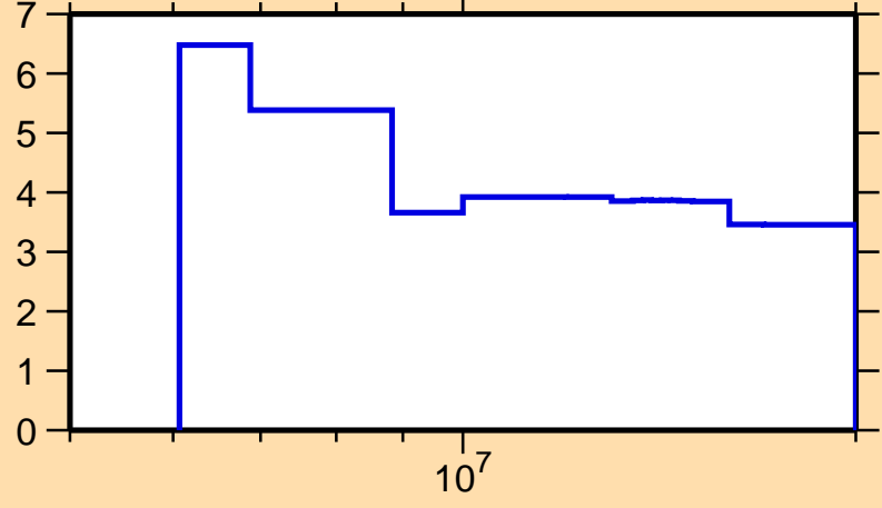
\Delta\sigma/\sigma vs. E for ^{192}\text{Os}(n,\text{tot.})
