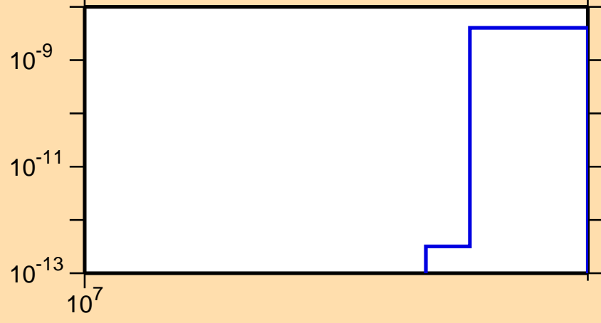
\sigma vs. E for ^{192}\text{Os}(n,\text{nd})
