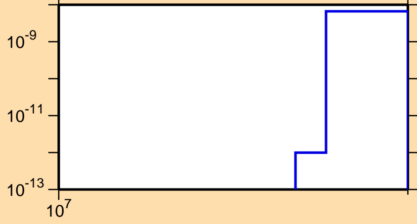
\sigma vs. E for ^{192}\text{Os}(n,nt)
