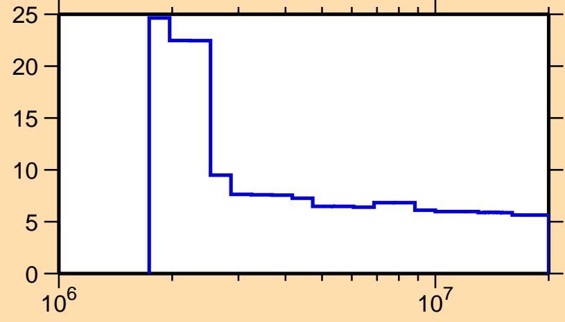
\Delta\sigma/\sigma vs. E for ^{192}\text{Os}(n,n\text{onel.})
