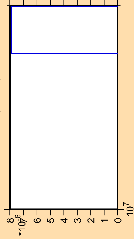
\Delta\sigma/\sigma vs. E for ^{192}\text{Os} (mt 11)
