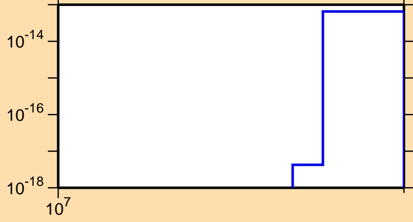
\sigma vs. E for ^{192}\text{Os}(n,\text{He}3)
