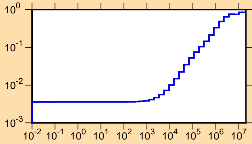
\mu vs. E for ^{192}\text{Os}(\text{mt251})
