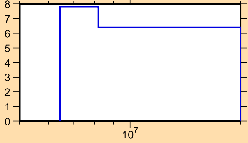
\Delta\sigma/\sigma vs. E for ^{192}\text{Os}(n,el.)
