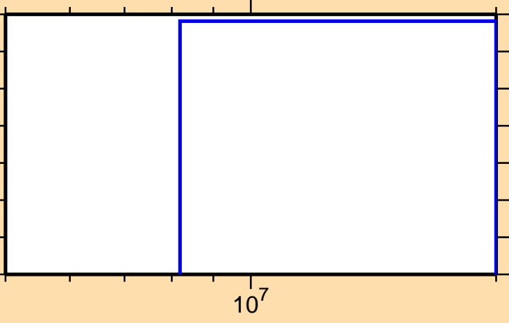
\sigma vs. E for ^{192}\text{Os}(n,3n)
