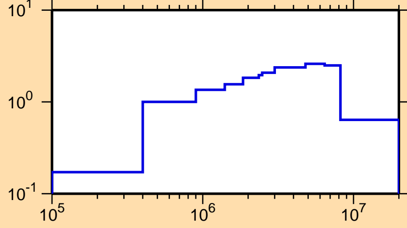
\sigma vs. E for ^{192}\text{Os}(n,\text{inel.})
