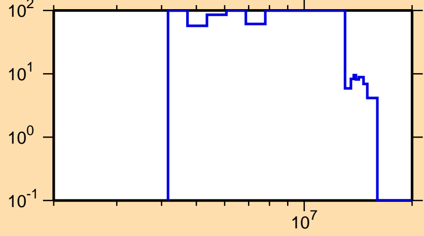
\Delta\sigma/\sigma vs. E for ^{192}\text{Os}(n,n_1)
