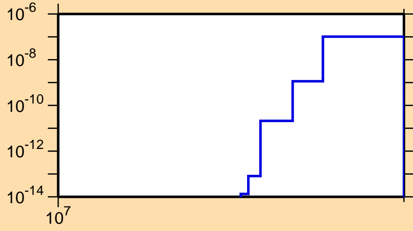
\sigma vs. E for ^{192}\text{Os}(n,nt)
