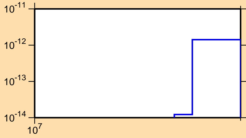
\sigma vs. E for ^{192}\text{Os}(n,\text{He}3)
