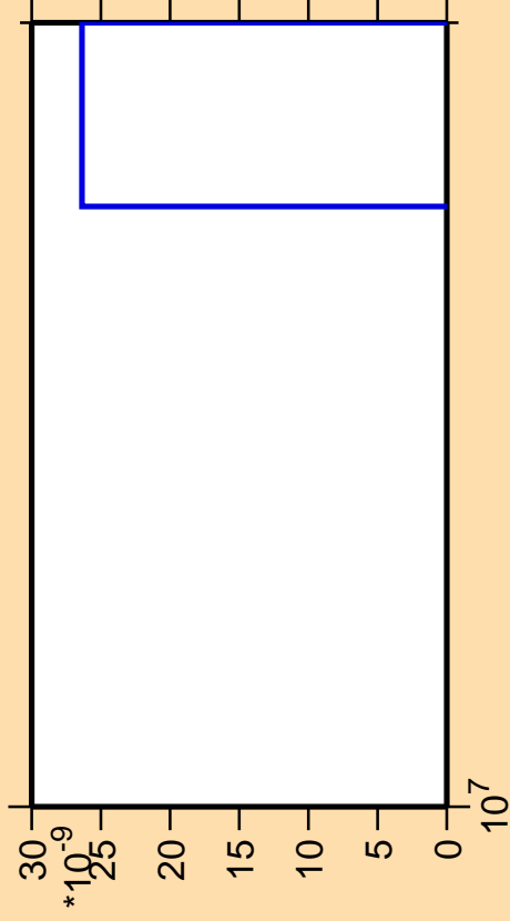
\Delta\sigma/\sigma vs. E for ^{193}\text{Os}(\text{mt } 11)
